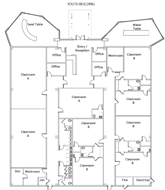
1/16" = 1'-0" YMCA YOUTH PROGRAM Concept Design 01/17/19 Copyright © Kinney Franke Architects AIA, Inc. 2018
